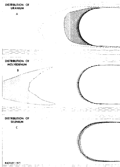
FIG. 4—Characteristic zoning of (A) uranium, (B) molybdenum, and (C) selenium in leading edge of geochemical cell. Intensity of hachuring is relative indication of concentrations which may range from traces to a few percent on same front.
