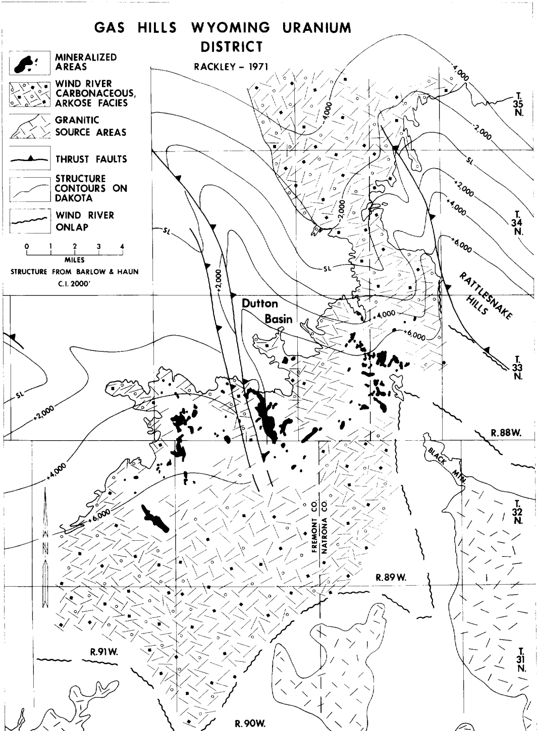
Fig. 9—Distribution of arkose facies and mineralized areas as presently known, shown on generalized structure map.
