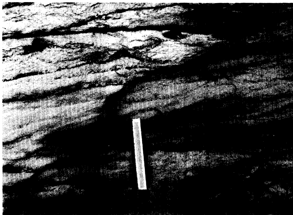
Fig. 2—Cross stratified arkose in sets 4-10 in. (10-25 cm) thick, with plant debris on cross-stratification surfaces, Shirley basin; scale is 12 in. (30.5 cm).
